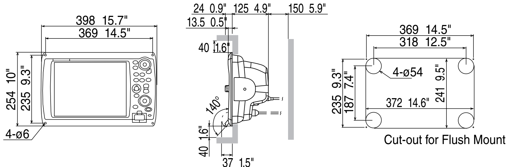
Multi Function Display (Flush Mount) MFD12
